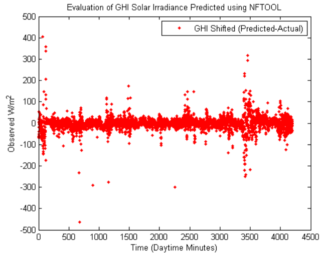
Figure 11. Best Neural Network GHI Error
