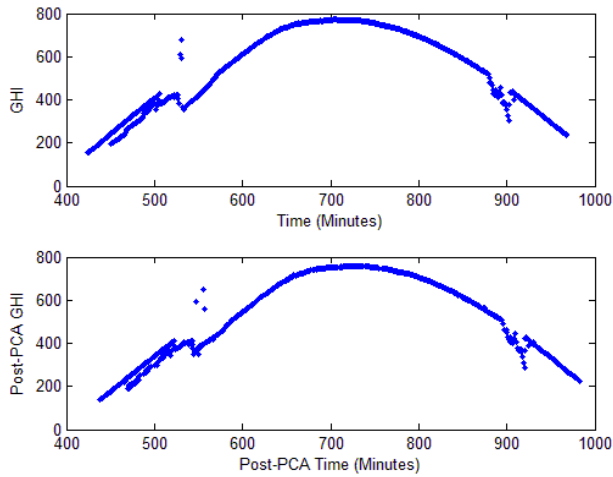
Figure 9. Data Recovery Demonstration Using First 50 Principal Components
