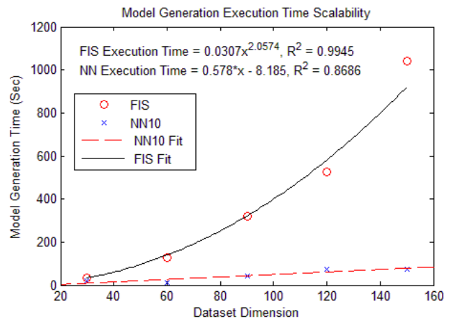
Figure 14. Model Generation Execution Time Relationship with Dataset Dimension
