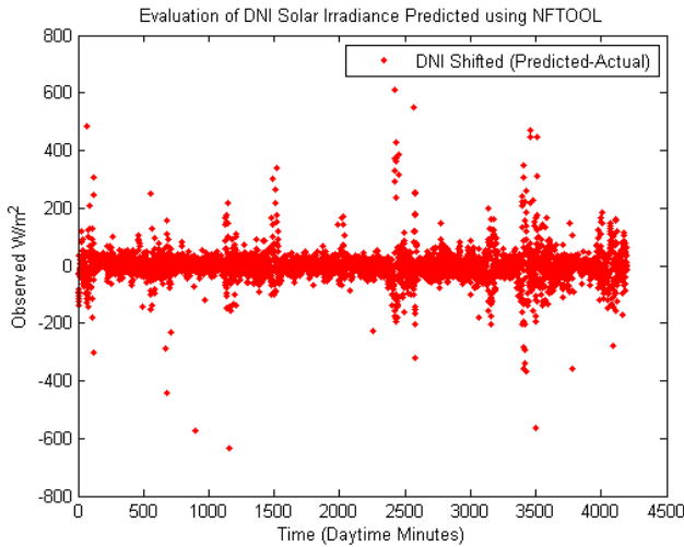
Figure 13. Best Neural Network DNI Error
