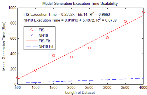
Figure 15. Model Generation Execution Time Relationship with Dataset Length
