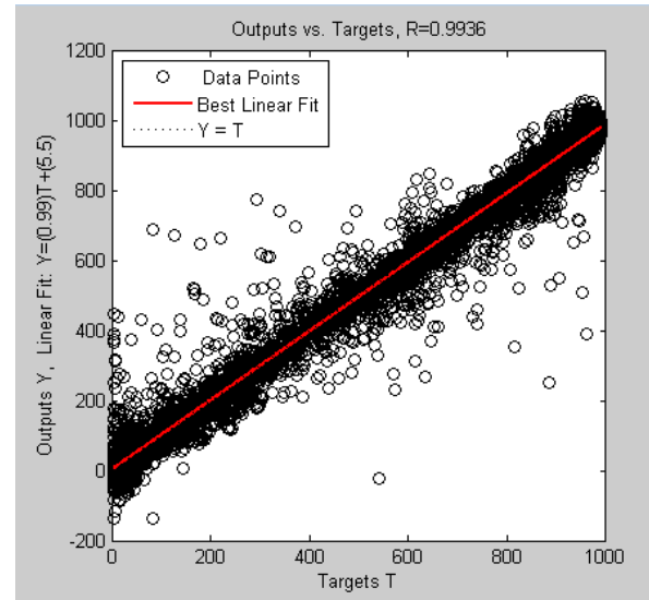
Figure 10. Best Neural Network Linear Regression Performance
