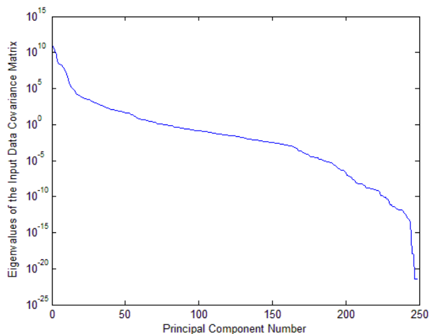
Figure 8. Principal Component Information Graph
