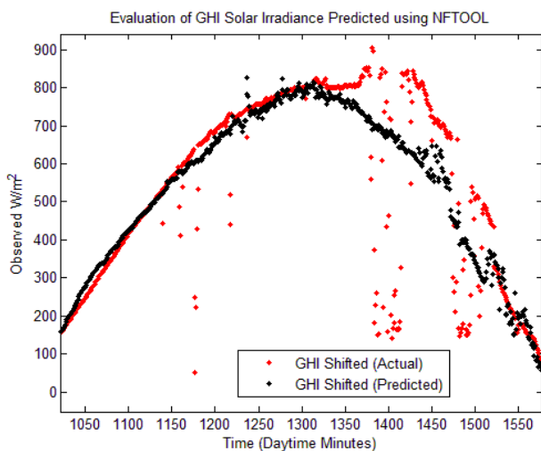
Figure 7. Data Generated Using NFTOOL Based on 13 Input Variables and 10 Hidden Neurons
