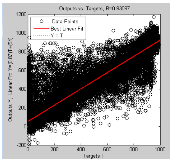
Figure 6. Post Training Network Regression Performance
