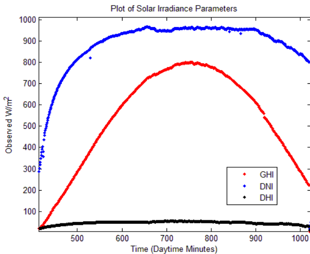
Figure 3. Three Key Irradiance Parameter Plot for a Clear Day
