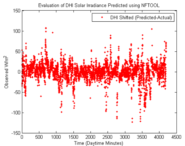
Figure 12. Best Neural Network DHI Error
