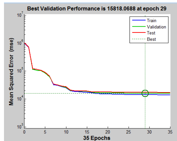
Figure 5. Back-propagation Performance Curve
