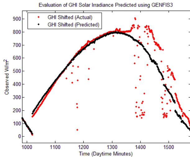
Figure 4. Data Generated Using GENFIS3 Based on 13 Input Variables
